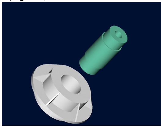
Figure 4 Trunnion to be slid through the hub after contracting.
