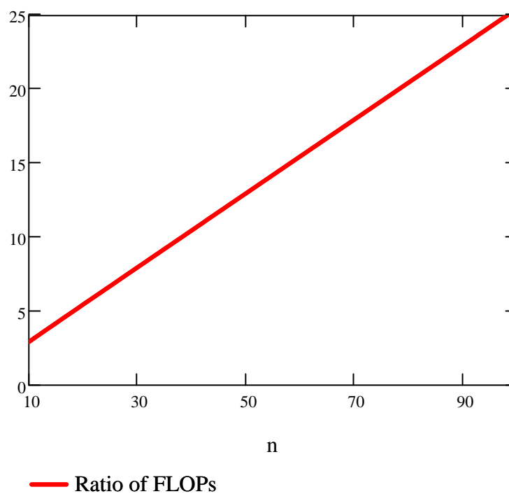
Ratio of Naive Gaussian Elimination FLOPs to LU Decomposition FLOPs
