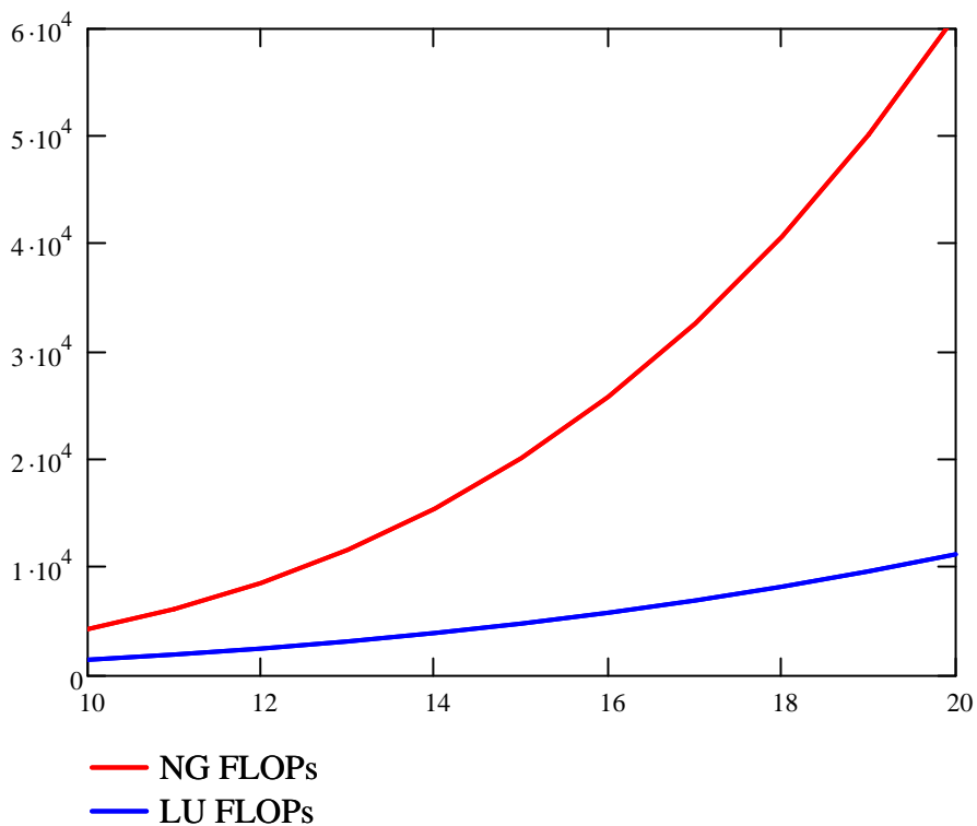
FLOPs for LU Decomposition and Gaussian Elimination versus Order of the Matrix
